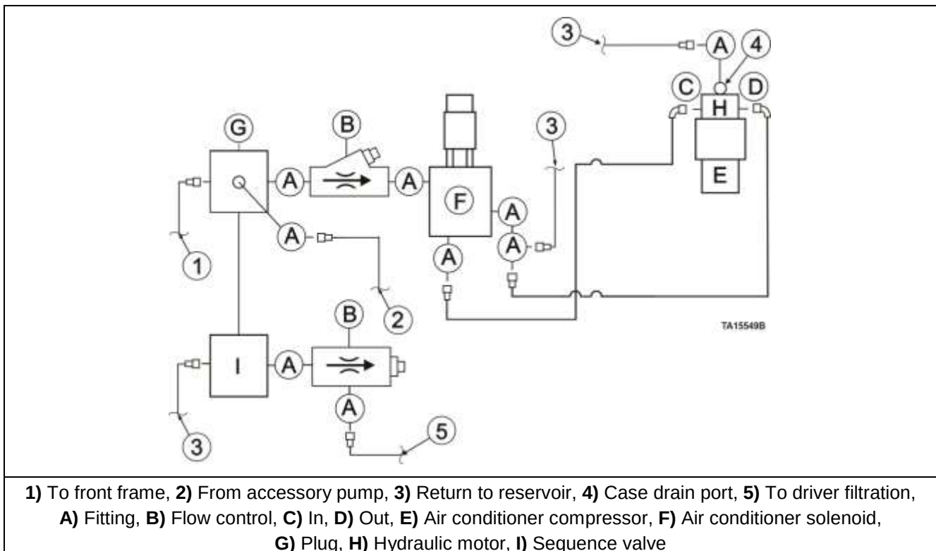
Figure 1. L-1350/L-1850/L-2350 air conditioning circuit
