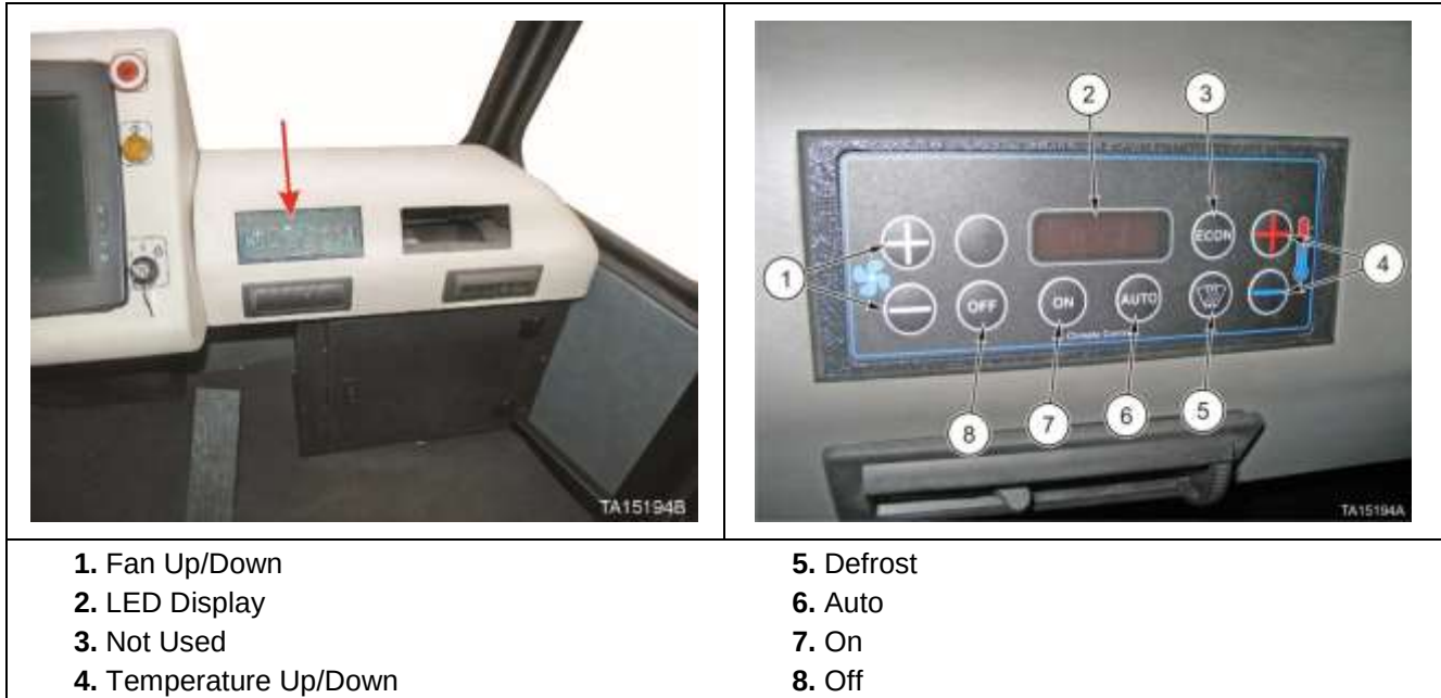
Figure 4. Climate control switches
