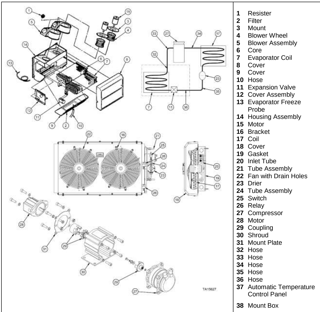
Figure 5. Air conditioner and heater assembly-typical
