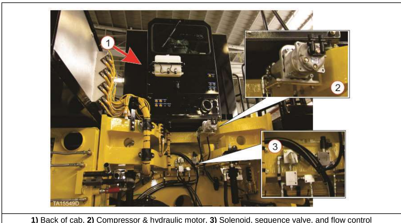
Figure 2. L-1350/L-1850/L-2350 air conditioner hydraulic component locations
