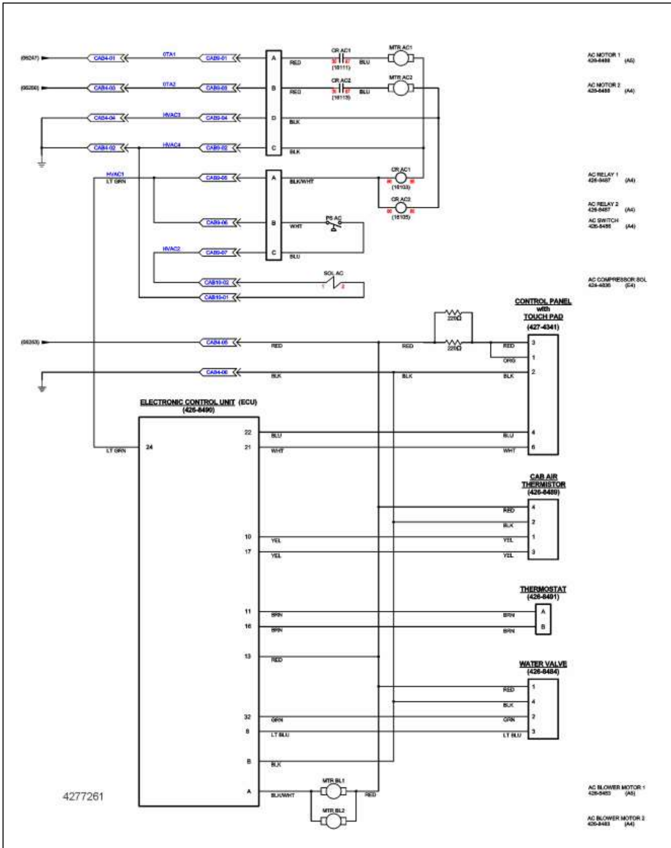
Figure 3. Air conditioning schematic (typical)
